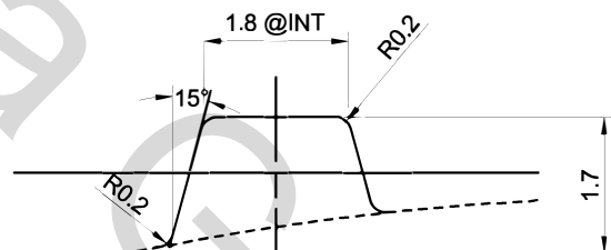
Details 'C' Scale 10:1
